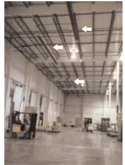
Loading dock area of warehouse heated with 28 ETS175's mounted 35' above finished floor.
